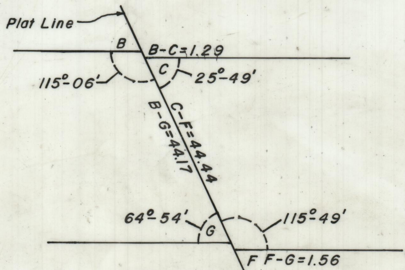
DETAIL Scale 1"=20'
